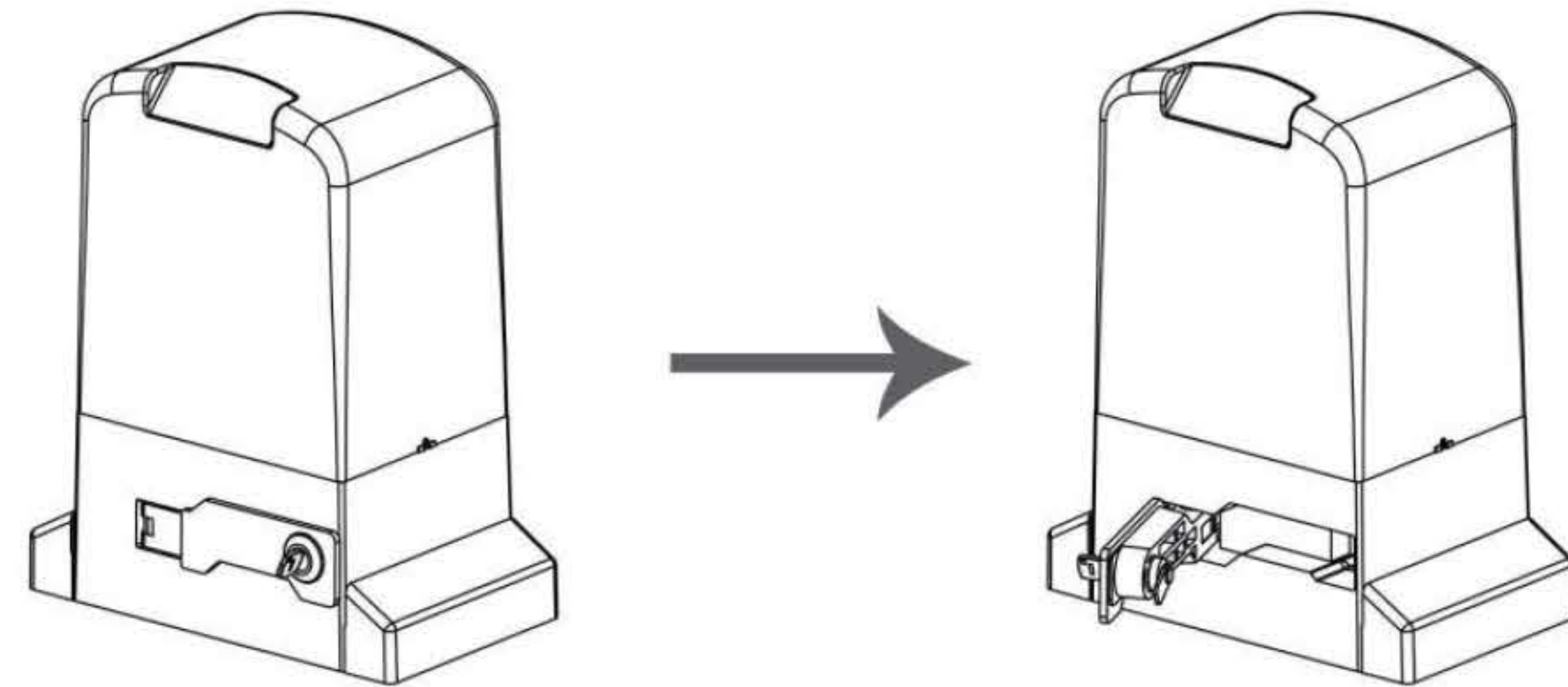
Releasing arm in torsion, wriggle 90 degree gate operator will be in releasing state
